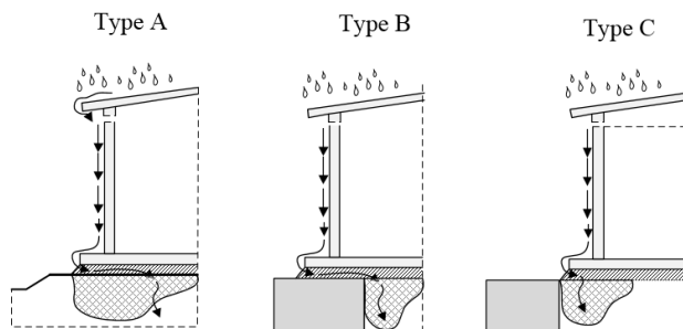
Figure 3: Penetration of rainwater under the bottom of tanks: Type A, Type B, Type C.
