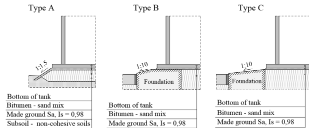
Figure 1: Analyzed types of tank foundations: Type A, Type B, Type C.
