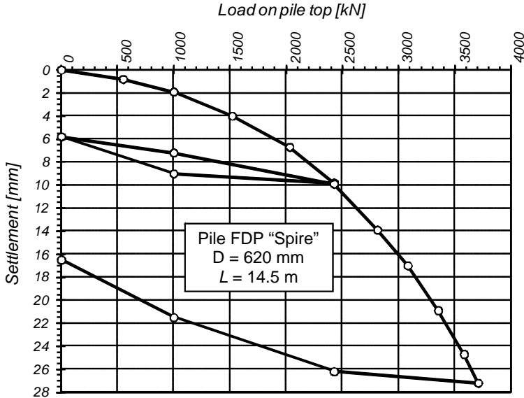
Fig. 1. An example of load–settlement curve resulting from static pile load test
