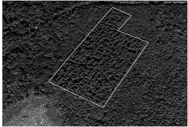
Figure 1. – Aerial photo of the test site taken in 1997. It is located in west-central Maine on an upland site (about 600 m above sea level) on a drumlinoid ridge underlain by a well-drained deep sandy loam soil. Precipitation ranges from 64–107cm and frost-free days from 80-145 days (USDA Natural Resources Conservation Services). There are 10 blocks, each with randomly located 3 tree plots representing each of the 51 families. The whole test is surrounded by a double border row of extra trees.
