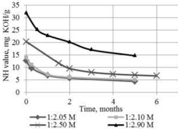
Fig. 4. Changes in NH groups during RO polyol's storage depending on time and RO:DEA molar ratio.
