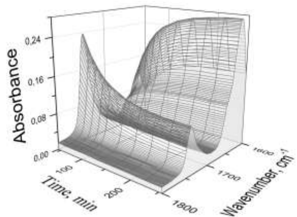
Fig. 7. Time resolved FTIR spectra during polyol's synthesis.
