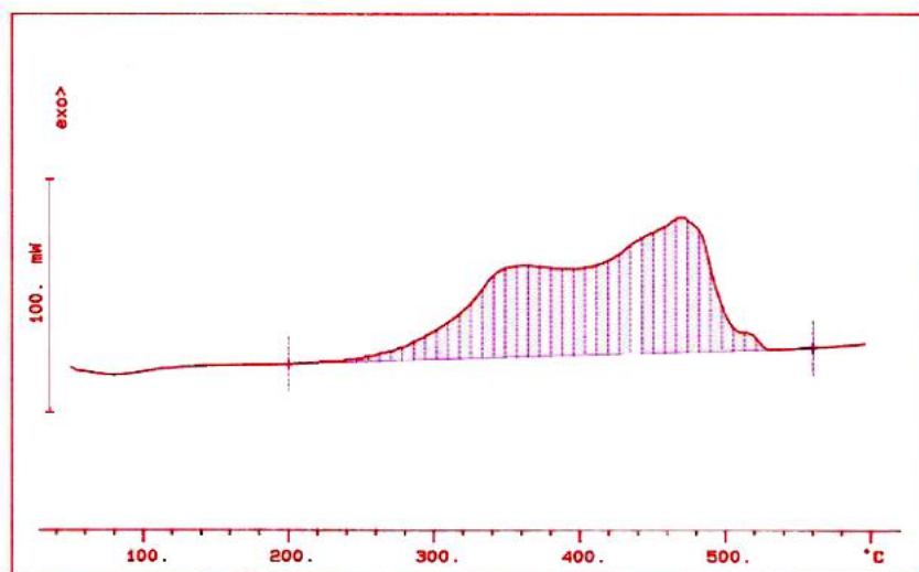
Fig. 6 DSC curve of thermal decomposition in nitrogen – sample B
