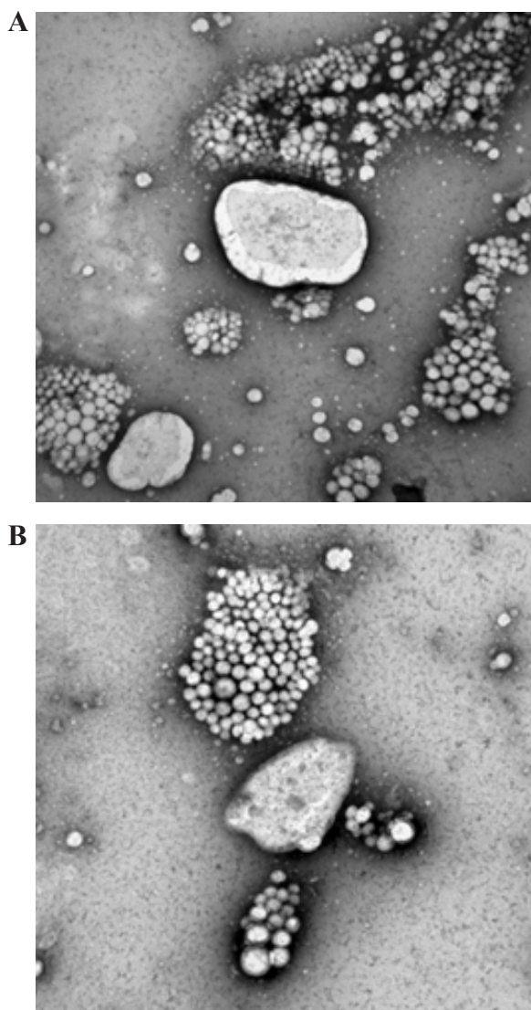
Figure 2. Transmission electron microscopy images (a) and (b) of sample after the \text{SnCl}_2 radiolabeling procedure ( \times 60k magnification)
