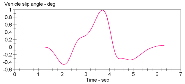
Fig.6. Sideslip angle curve.
