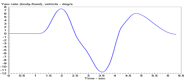
Fig.5. Yaw rate curve.
