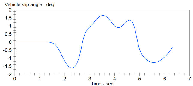
Fig.8. Sideslip angle curve.
