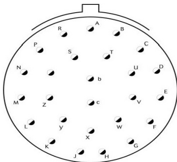
Fig.11. Sensor connector.
