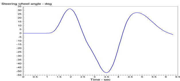
Fig.4. Steering wheel angle input curve.
