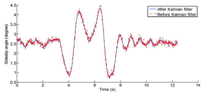
Fig.19. Sideslip angle curve.
