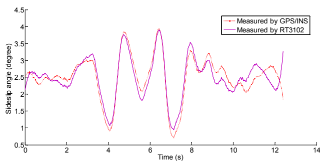
Fig.20. Sideslip angle curve measured by RT3102 sensor.
