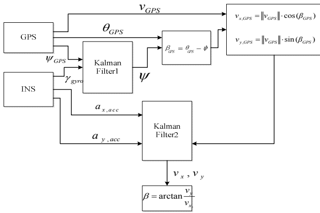
Fig.2. Sideslip angle combination algorithm block.
