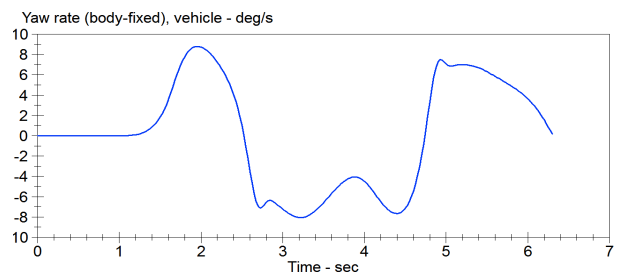
Fig.7. Yaw rate curve.
