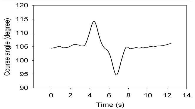
Fig.17. Course angle curve.
