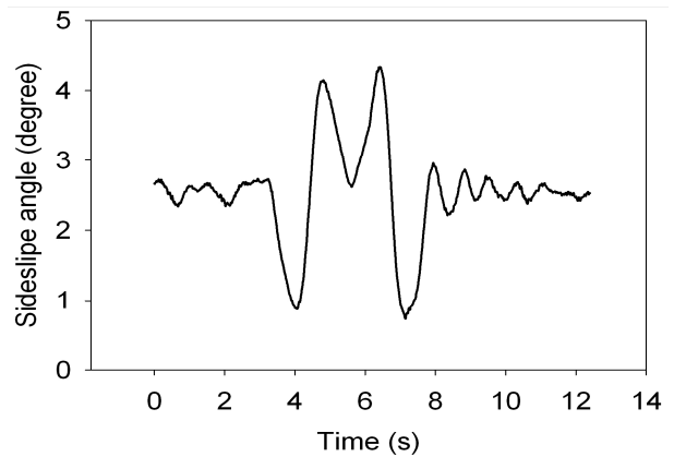
Fig.18. Sideslip angle curve.
