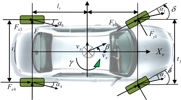
Fig.1. Eight DOF vehicle dynamic model.
