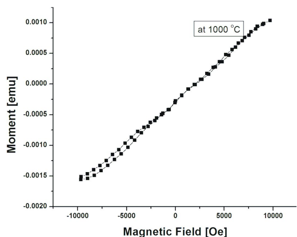
Fig. 5. Magnetic properties of NiO nanoparticles after annealing at 1000 °C.
