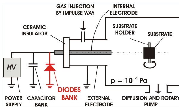
Fig. 1. Schematic diagram of the IPD device equipped with diodes bank.
