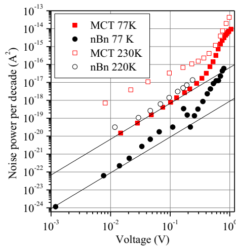
Fig. 9. Averaged power per decade of the low frequency noise P_{\text{dec}} calculated with formula (7) for nBn (points) and MCT detectors (squares) at 77 K (filled symbols) and 220 K/230 K (empty symbols) as a function of bias voltage. Black solid lines have the slope of two.
