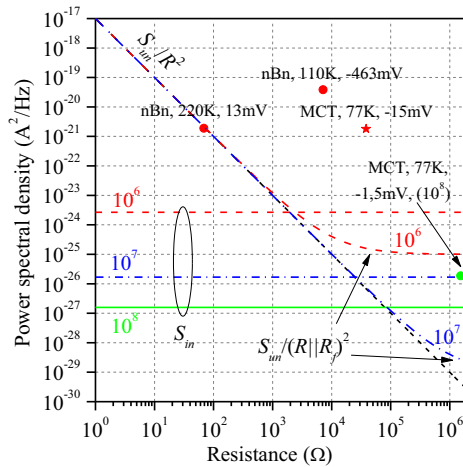
Fig. 5. Background noise components S_{in}/R^2 , S_{in}/(R||R_i)^2 and S_{in} at f = 100 Hz versus dynamic resistance R of the photodetector. Colors/line styles refer to different transimpedance gain k_{iu} = 10^6 (red/dashed), 10^7 (blue/dashed-dotted), 10^8 (green/solid). Dots and star represent measured values of S_i(f = 100 Hz). Device, temperature, bias and gain (unless 10^6 ) are given for each measurement.
