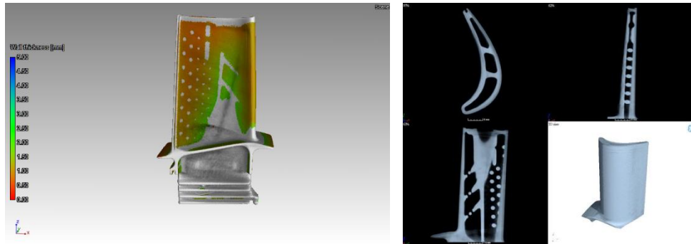
Fig. 1. Tomograms of turbine blades showing: thickness of turbine blade walls (left), internal blade walls [2]
