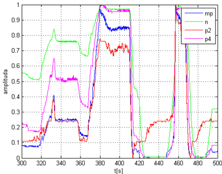
Fig. 3. Plots of standardised signals from turbojet engine's automatic control system (mp – standard, n – rotational speed, p – pressures)
