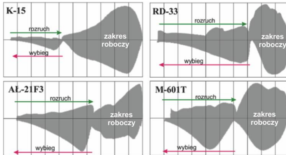
Fig. 4. Phase portraits for rotational speeds of engines
