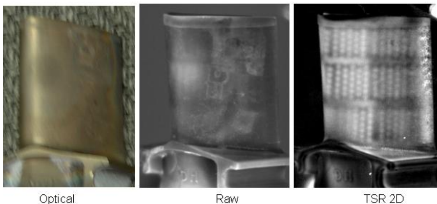
Fig. 2. Images of a high-pressure turbine blade examined with different methods: an optical method, RAW, TSR 2D [3]
