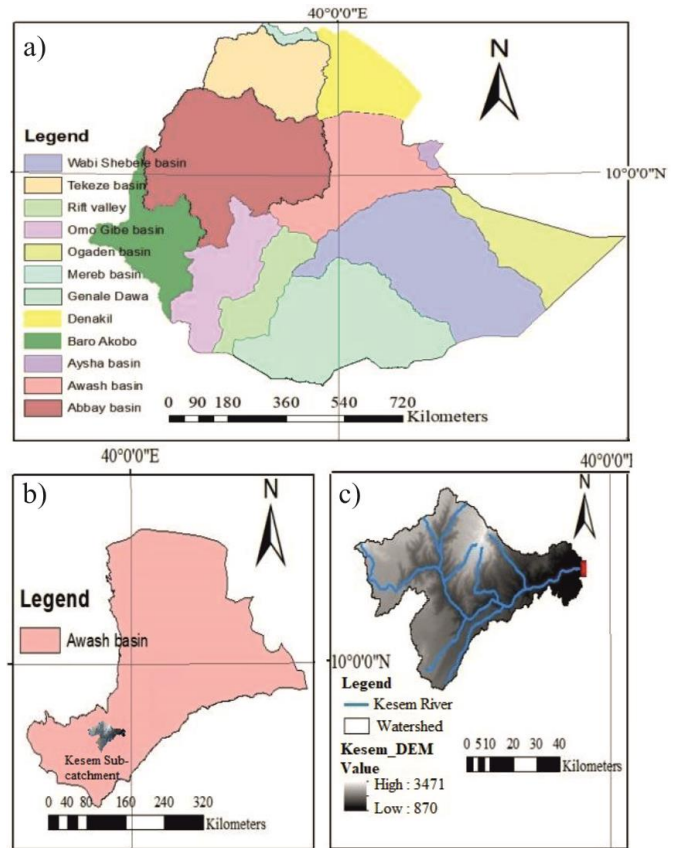
Fig. 2 a) Ethiopia River basins, b) Awash basin, c) Kesem sub-catchment
