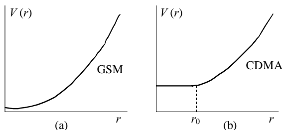
Fig. 2. Models of BS power control: (a) — monotonically increasing power as the function of distance, (b) — monotonically nondecreasing function (users at the distance r \leq r_0 receive power as if they are on the distance r_0 )
