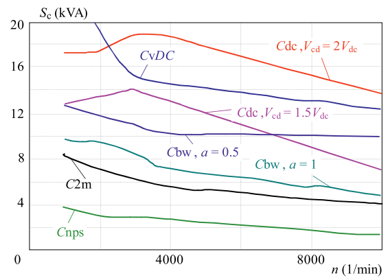
Fig. 20. Apparent power vs speed for investigated SRG converters
