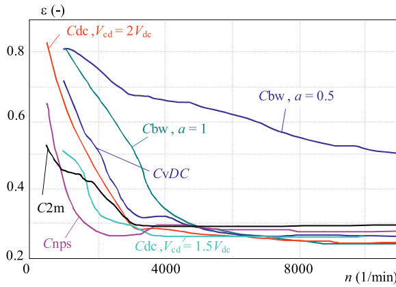
Fig. 22. Excitation factor vs speed for investigated SRG converters
