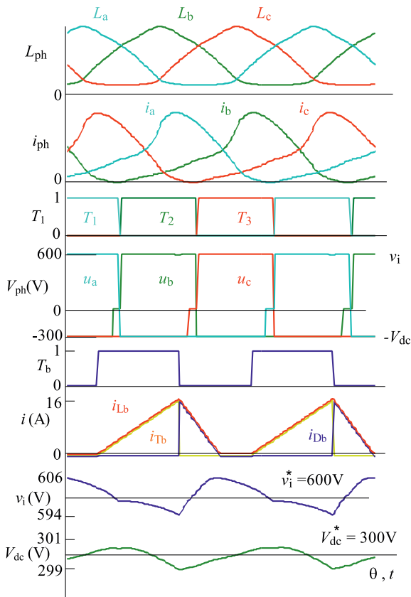
Fig. 18. Simulated waveforms of the three phase 12/8 SRG converter with variable DC link, v_i = 2V_{dc} = 600 V and n = 10000 rpm.
