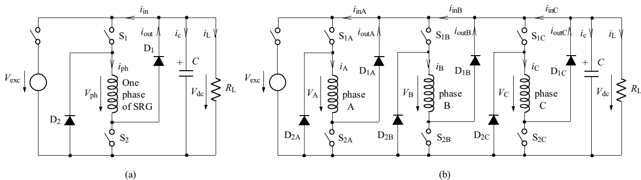
Fig. 3. Equivalent circuit of 2m converter in (a) – single phase, (b) – three phase operation
