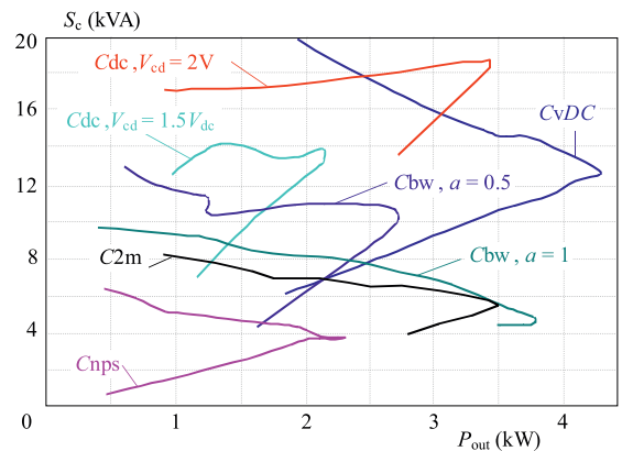
Fig. 21. Apparent power vs output power for investigated SRG converters
