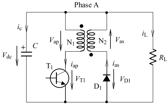
Fig. 14. Equivalent circuit of the converter with bifilar winding
