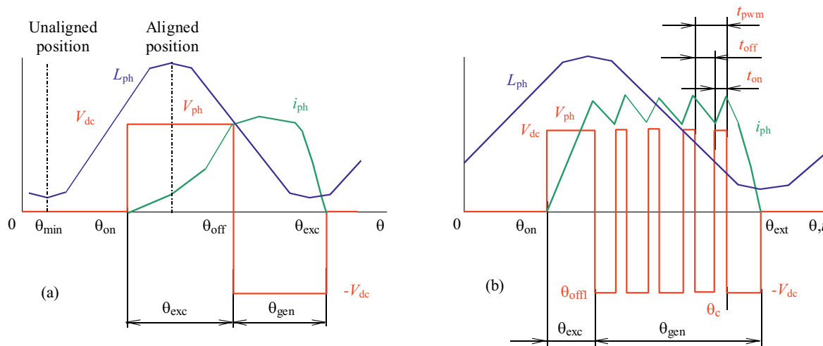
Fig. 1. SRG phase variables at: (a) – single pulse operation, (b) – multi-pulse operation, current control
