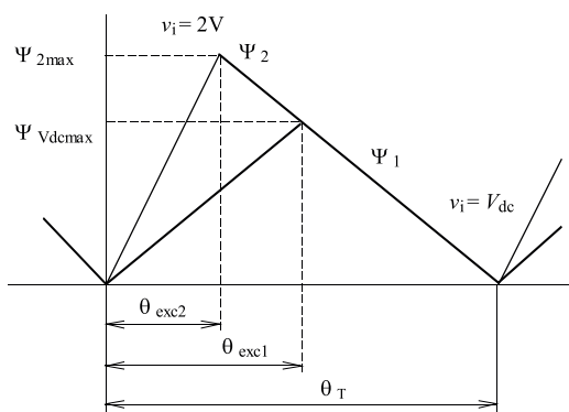
Fig. 24. Waveforms of linkage magnetic flux of the SRG with converter with variable DC link at v_i = v_{dc} (\psi_1) , and v_i = 2v_{dc} (\psi_2)
