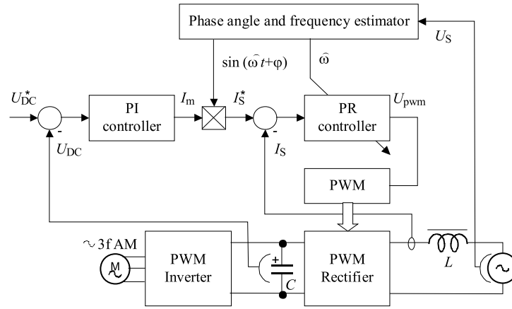
Fig. 3. Control structure of a single phase PWM rectifier
