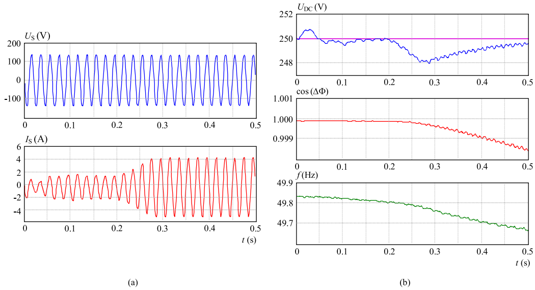
Fig. 8. Transient responses (PWM rectifier and inverter): short-circuit AM in t_s = 0.2 s; a) input voltage and current, b) DC-link voltage, power factor and frequency
