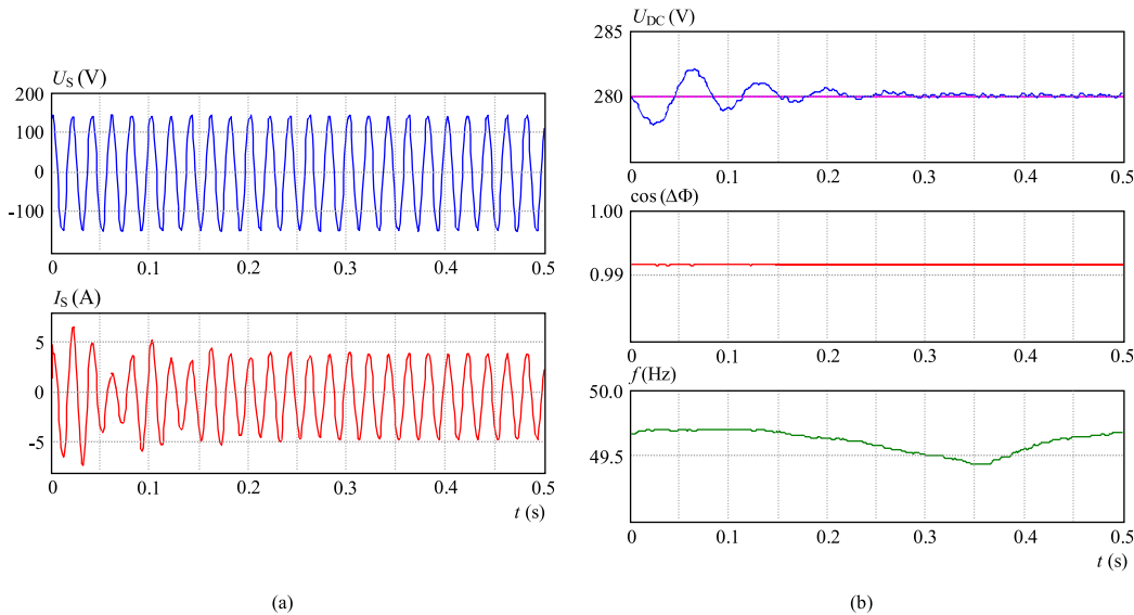
Fig. 7. Transient responses (PWM rectifier and inverter): no-load AM; a) input voltage and current, b) DC-link voltage, power factor and frequency
