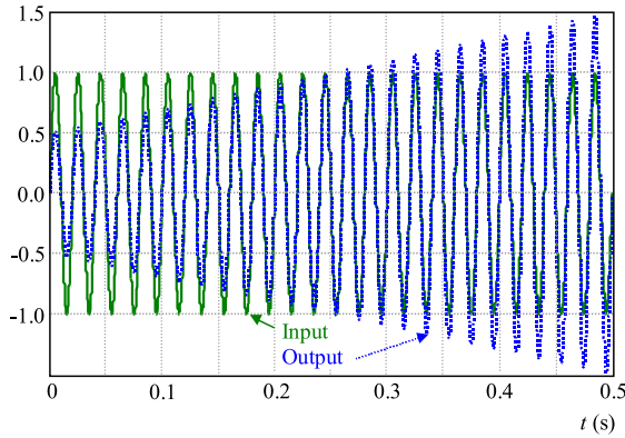
Fig. 4. Time domain response of the PR controller
