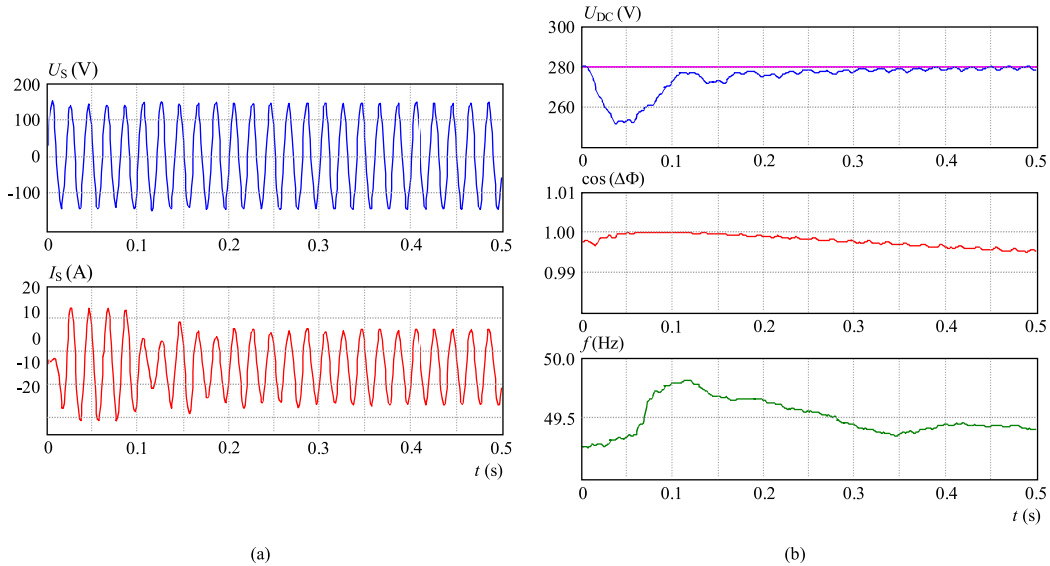
Fig. 9. Transient responses (PWM rectifier and inverter): load on AM; a) input voltage and current, b) DC-link voltage, power factor and frequency
