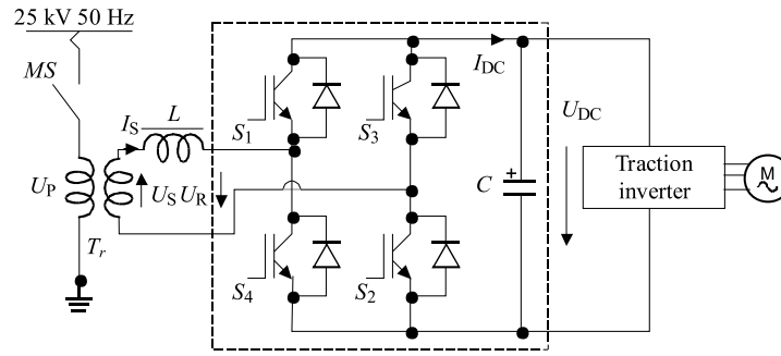
Fig. 1. Structure of a single phase PWM rectifier
