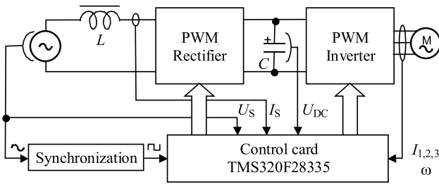
Fig. 5. Simplified block diagram of the PWM rectifier
