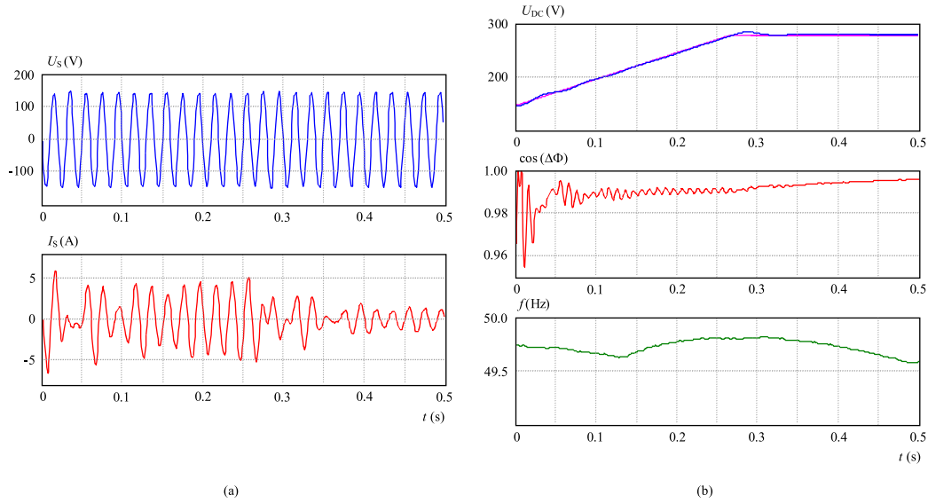
Fig. 6. Transient responses when DC-link voltage changes gradually with no-load; a) input voltage and current, b) DC-link voltage, power factor and frequency
