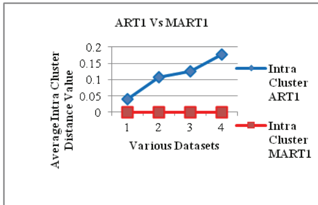
Figure 3. ART1 Vs MART1 intra-cluster distance
