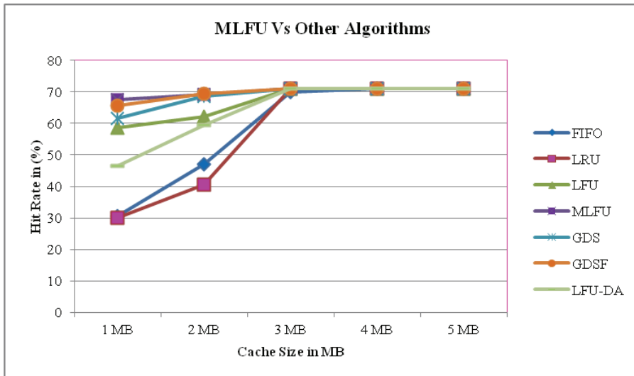
Figure 7. Comparison of Hit Rate by FIFO, LRU, LFU and MLFU on Dataset (sv[1].sanitized-access.20070109)
