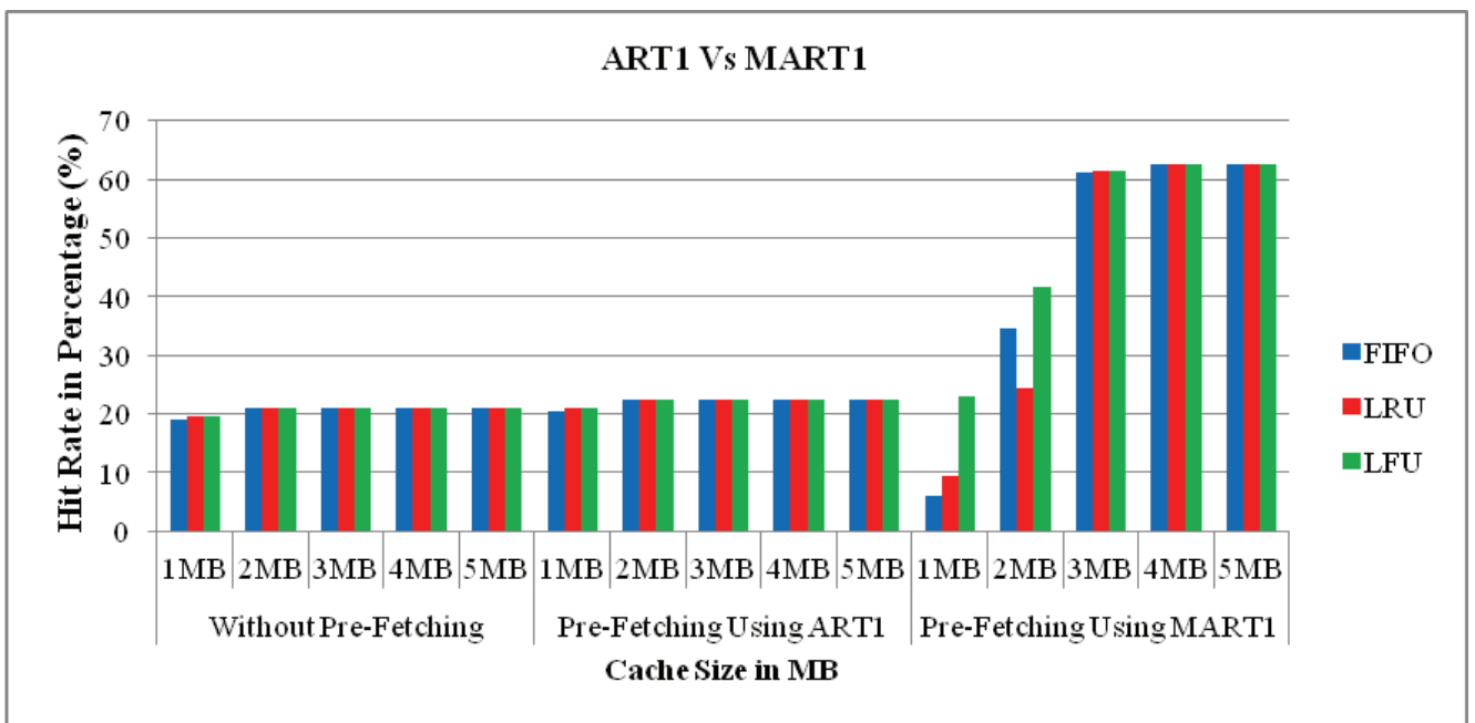
Figure 5. ART1 Vs MART1 using Data Set (ny[1].sanitized-access.20070109)
