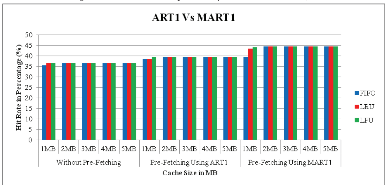
Figure 6. ART1 Vs MART1 using Data Set (bo2[1].sanitized-access.20070109)
