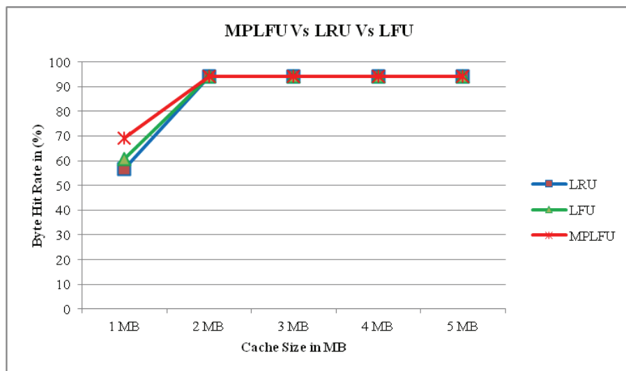
Figure 8. Byte Hit Rate of LRU Vs LFU Vs MPLFU on dataset (bo2[1].sanitized-access.20070109)
