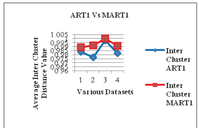
Figure 4. ART1 Vs MART1 inter-cluster distance
