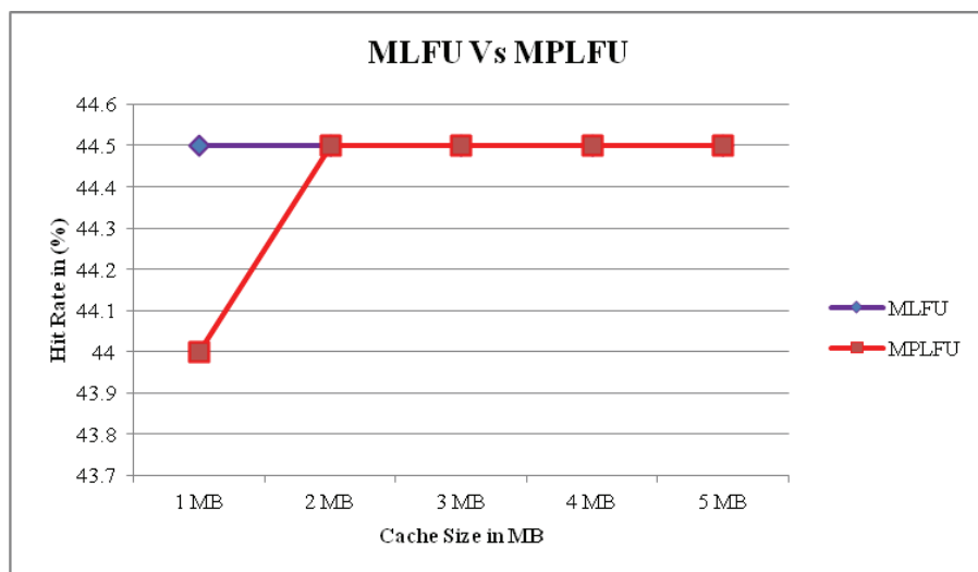
Figure 9. Comparison of Hit Rate in MLFU and MPLFU on dataset (uc[1].sanitized-access.20070109)
