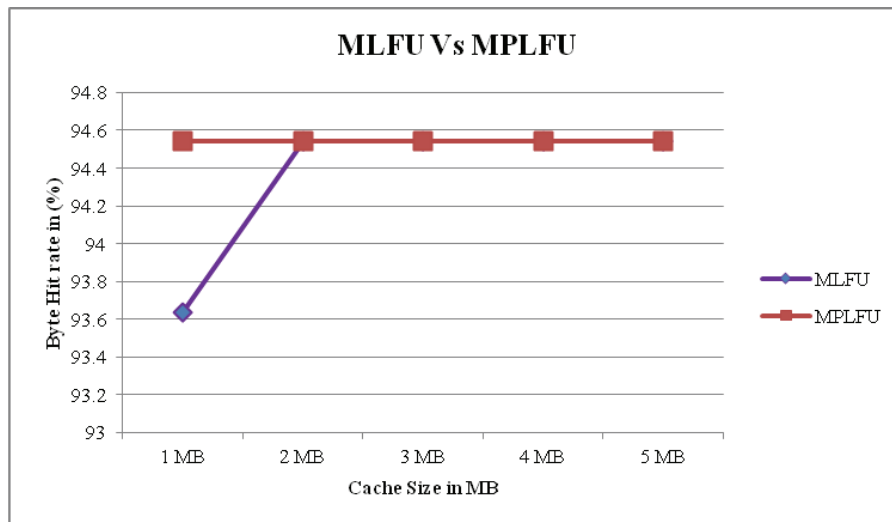
Figure 10. Comparison of Byte Hit Rate in MLFU and MPLFU on dataset (uc[1].sanitized-access.20070109)
