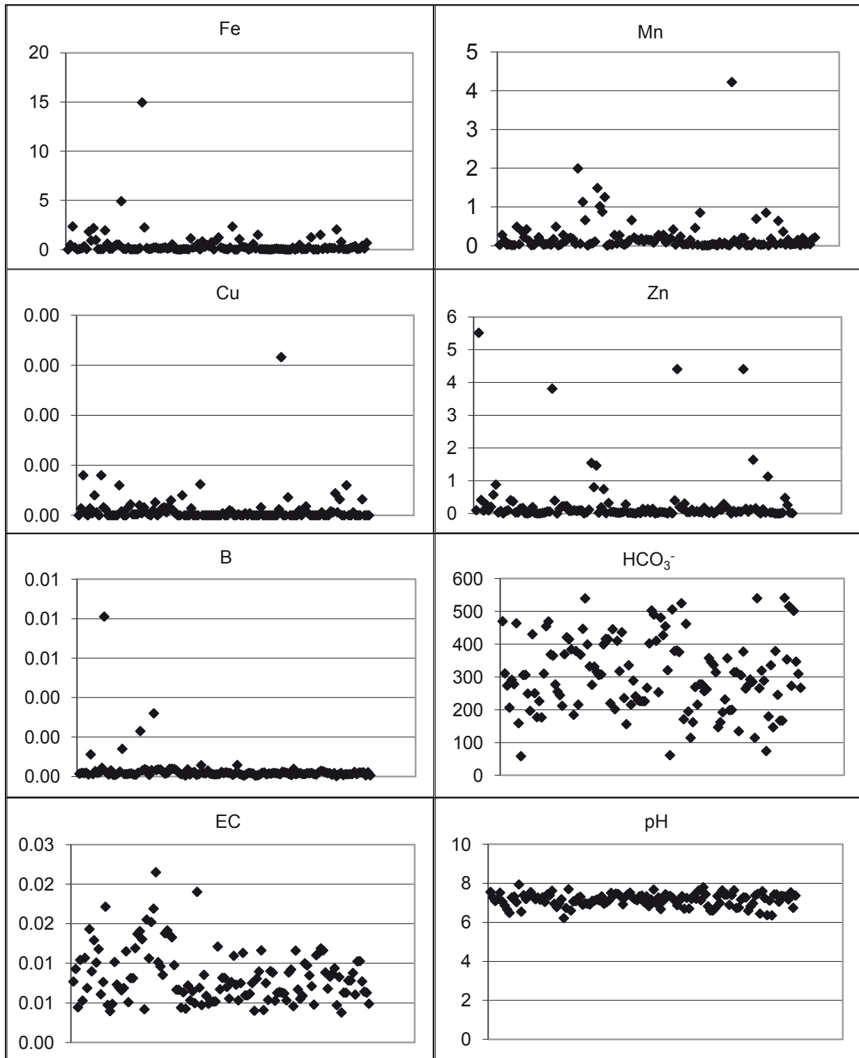
Figure 2. Chemical composition of water samples ( \text{mg dm}^{-3} ), EC ( \text{mS cm}^{-1} ) and pH
