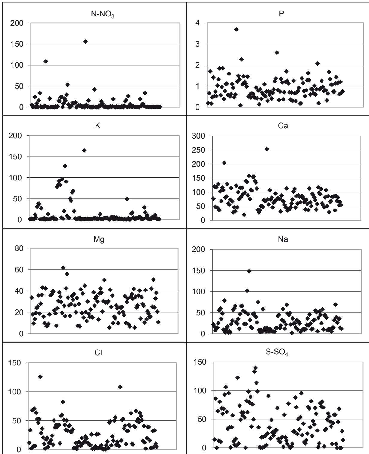
Figure 1. Chemical composition of water samples ( \text{mg dm}^{-3} )
