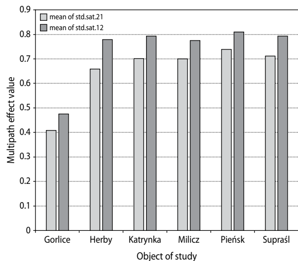
Figure 5. Values of standard deviation for a single satellite and L1 and L2 frequencies with respect to the object of study
