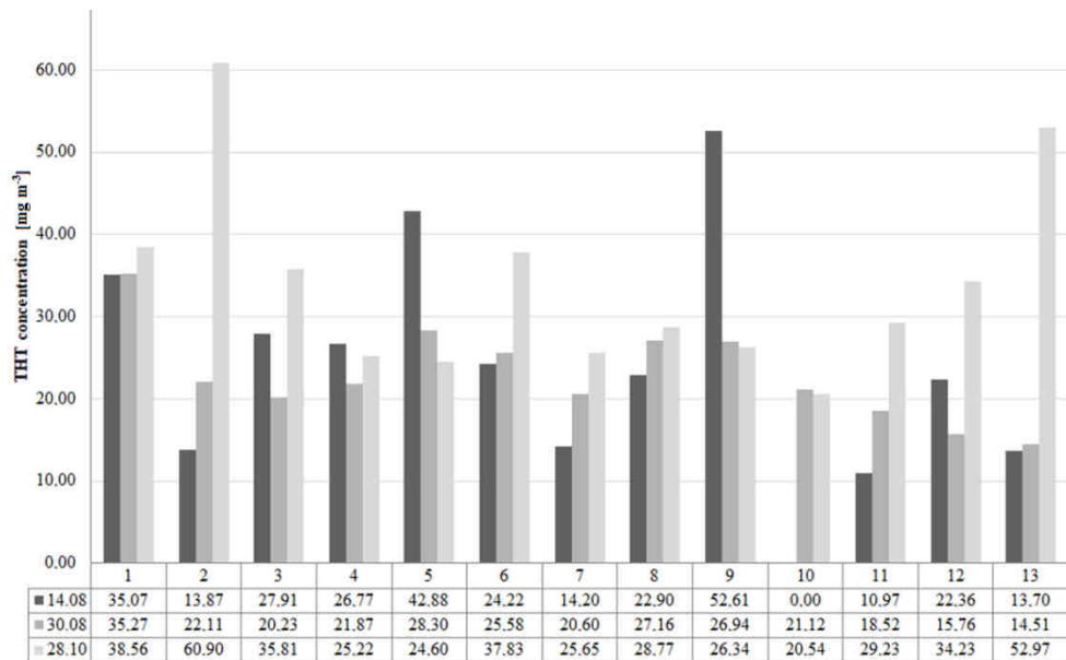
Fig. 3. Results of THT concentration in 3 series, in 13 measuring points
