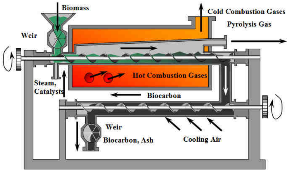
Fig. 2. Scheme of plate device for thermal decomposition of biomass working continuously [13]
