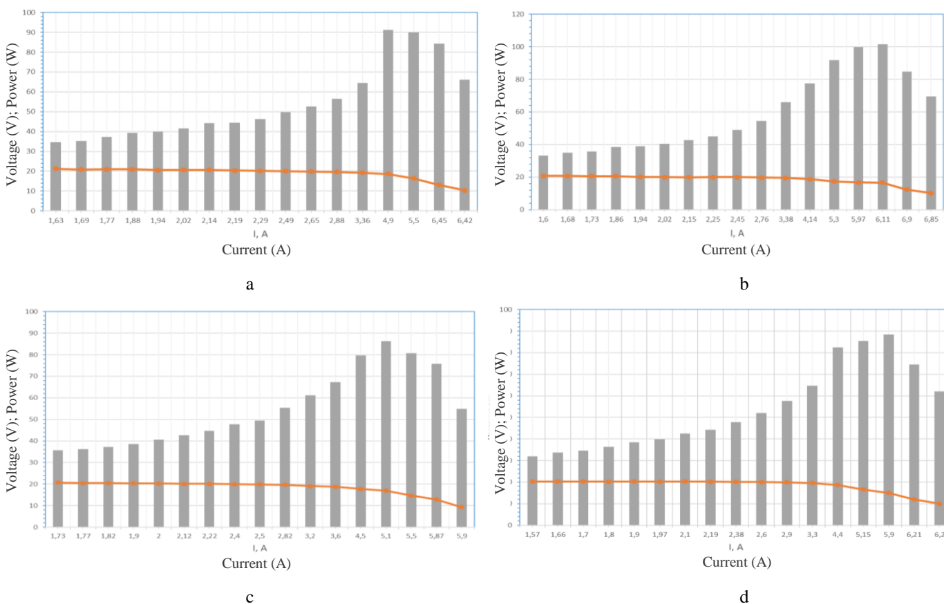
Fig. 4. Volt-ampere and load characteristics of the PV panel: a, b – polycrystal; c, d – monocrystal.
