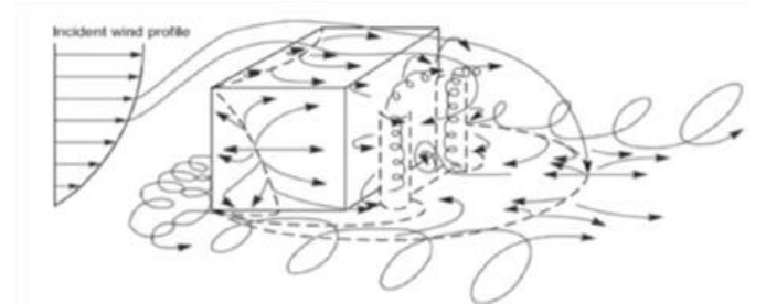
Fig. 6. 3-D wind flow around the rectangular box [17].
