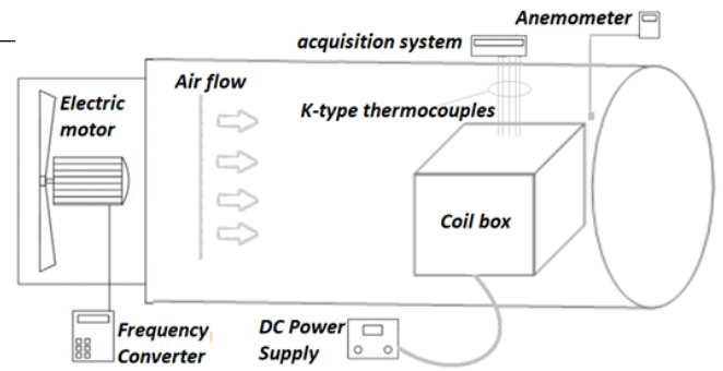
Fig. 4. Schematic diagram of the main part of the experimental setup.
