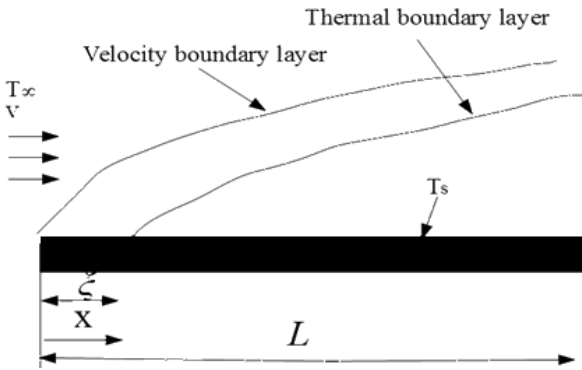
Fig. 1. Illustration of the coolant flows over a flat plate with an unheated part.
