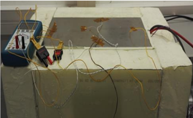
Fig. 3. The used configuration for the flat plate experiment.
