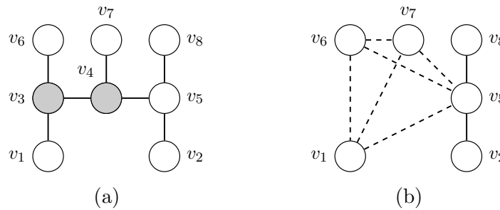
Figure 2. A graph and its reduction by \{v_3, v_4\} .
