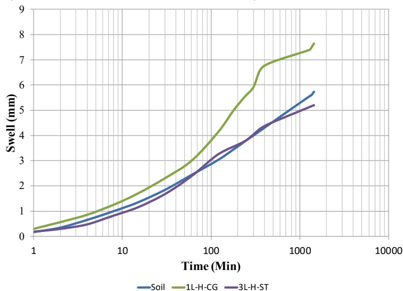
Fig. 10. Swell of Soil Embedded with 1 Layer of CG and 3 Layers of ST
