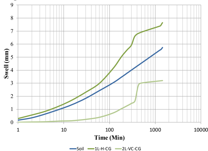
Fig. 12. Swell of Soil Embedded with 1 Horizontal Layer and 2 Vertical Cross Layers of CG
