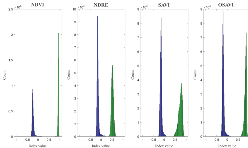
Figure 3. Histogram of the statistical distribution of the Vegetative Indexes for the selected area covered by vegetation (green histogram) and water (blue histogram). To distinguish between vegetation and water bodies, the procedure will select the most useful vegetative index, which has the biggest difference between the two distributions. In this way, a clear classification is expected.
