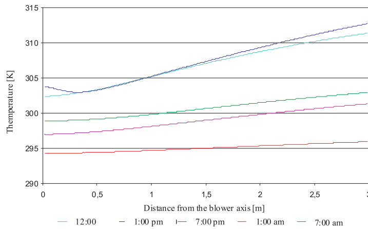
Figure 8. Sludge surface temperature as a function of the distance from the blower axis for various times of the modelled day.
