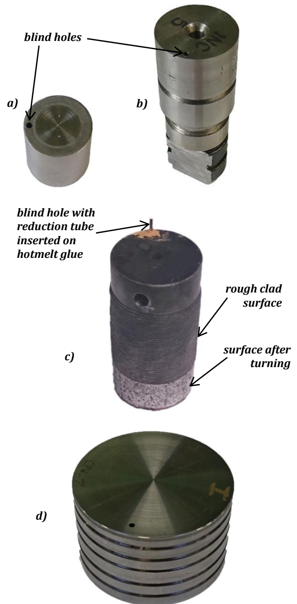
Fig. 1. View of tested samples used in research: a) Inconel 625, b) Inconel 718, c) WC-Co, d) Waspaloy
