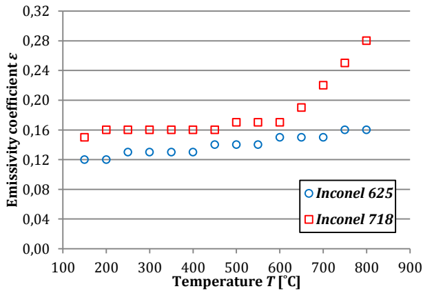
Fig. 7. Emissivity coefficient according to temperature for Inconel 625 and Inconel 718
