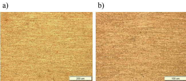
Fig. 2. Microstructure of the base metal (BM) of the 5.0 mm thick S700MC steel sheet at different magnification, 3% Nital etched, Table 1
