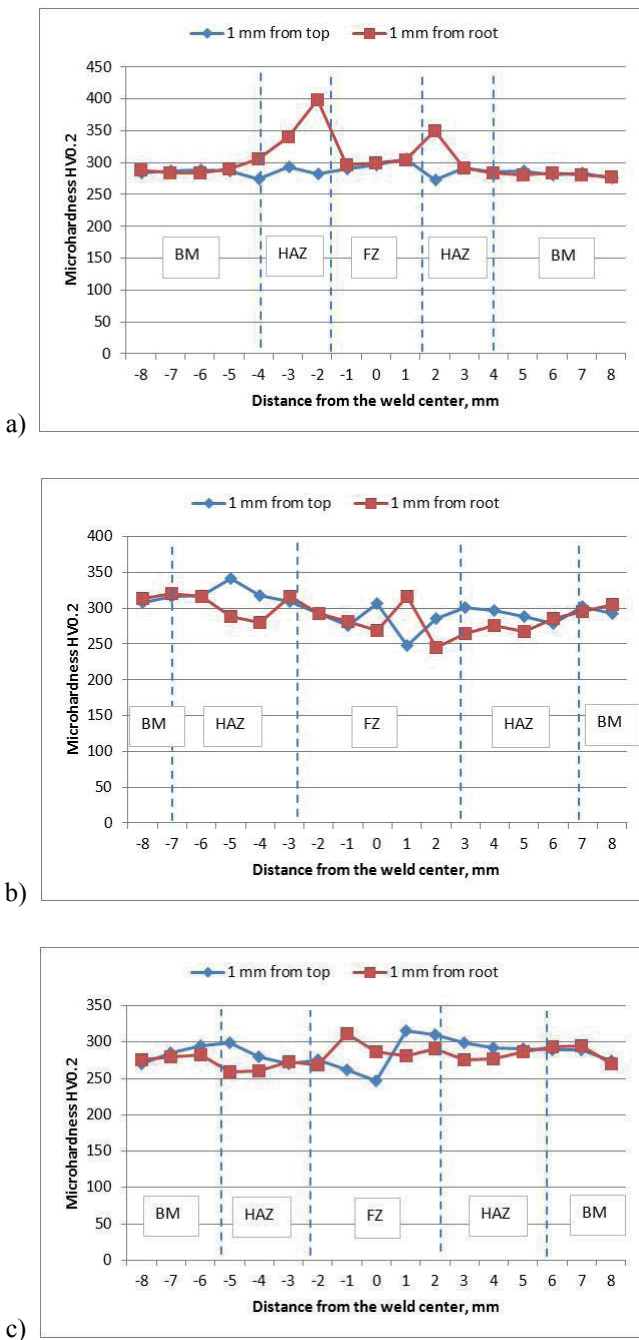
Fig. 7. Microhardness distribution (profile) across the 5.0 mm thick butt joint of S700MC steel plate autogenously welded by the disk laser (Table 4); a) joint A, b) joint B, c) joint C
