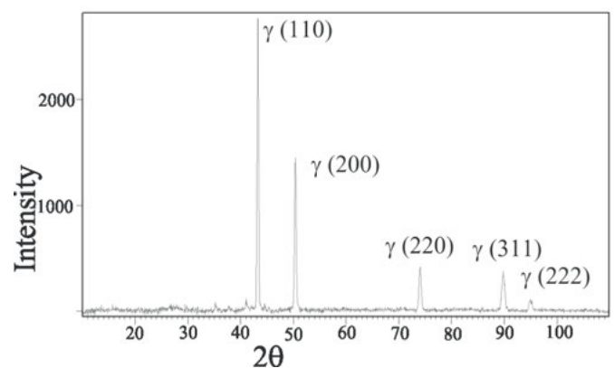
Fig.7. X-ray diffractogram of the Inconel 625 weld overlay
