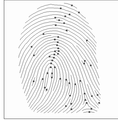
Fig. 9. Fingerprint sample, where points with the highest ridge curvature are indicated by means of Algorithm A2.
