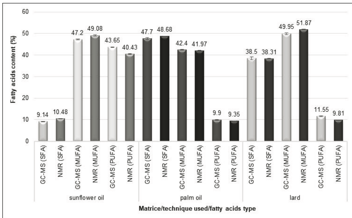
Figure 4. Comparative content (mean \pm SD,%) in SFA/MUFA/PUFA determined by GC-MS and NMR from the investigated food matrices
