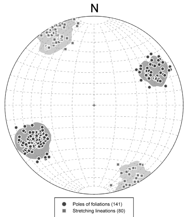
Figure 4: Stereographic plots of the mylonitic foliation with 5% contours indicated and the stretching lineations. The software InnStereo Beta 5 ( http://innstereo.github.io/ ) was applied for preparing stereoplots.
