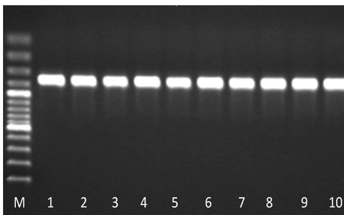
Figure 1. Electrophoretic separation of PCR products with VP1 primers in 1% agarose gel. A distinct band of about 380 bp was obtained. M – size marker 100bp (with brighter bands 500 bp and 1000bp) , 1-10 – test samples
