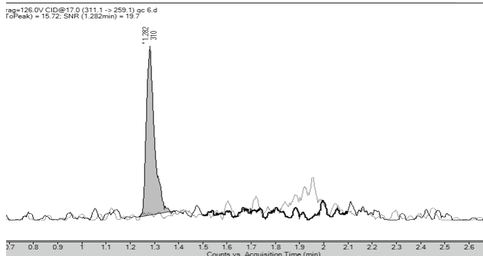
Fig. 2. A typical chromatogram of desloratadine obtained with liquid chromatography with tandem mass spectrometry (LC-MS/MS).
