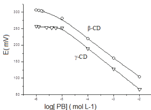
Fig. 4. Calibration curve of phenobarbitone membrane sensors (in 10^{-2} mol L -1 sodium sulphate). Calibration curve equations for \beta - (sensor 1) and \gamma -CD (sensor 2) are: y = -59.1x - 15.1 and y = -62.0x - 51.6 , respectively.
