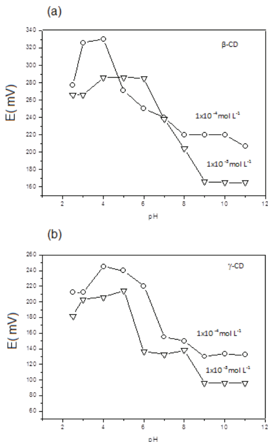
Fig. 3. pH profile of phenobarbitone sensors: a) sensor 1 with \beta -CD and b) sensor 2 with \gamma -CD, using: 1 \times 10^{-3} (empty triangles) and 1 \times 10^{-4} (empty circles) mol L -1 phenobarbitone.
