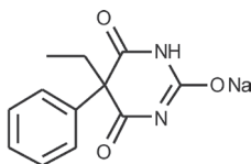
Fig. 1. Chemical structure of phenobarbitone sodium, C_{12}H_{11}N_2NaO_3 , M_r 254.22.
