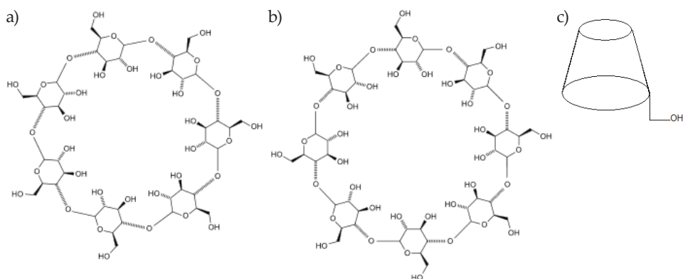
Fig. 2. Chemical structure of: a) β-cyclodextrine, b) γ-cyclodextrine, c) toroidal shape.
