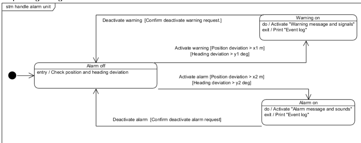
Figure 10: The state machine diagram for handling alarm unit of DP-system
