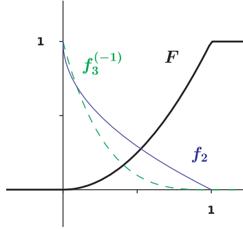
FIGURE 4. Illustration of Example 3 with non-invertible case n = 3 .
