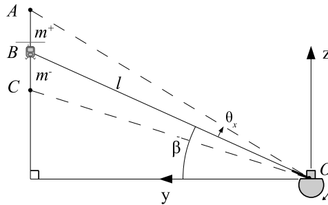
Fig. 6. Diagram of deviation formation as a result of side tilting of the ship, where: l = |OB| — target distance, m^+ = AB — missing over the target, m^- = -|BC| — missing under the target, \beta — cannons' lifting angle (elevation), \theta_x — directed tilt angle of a moving object (ship) around axis x [own work]
