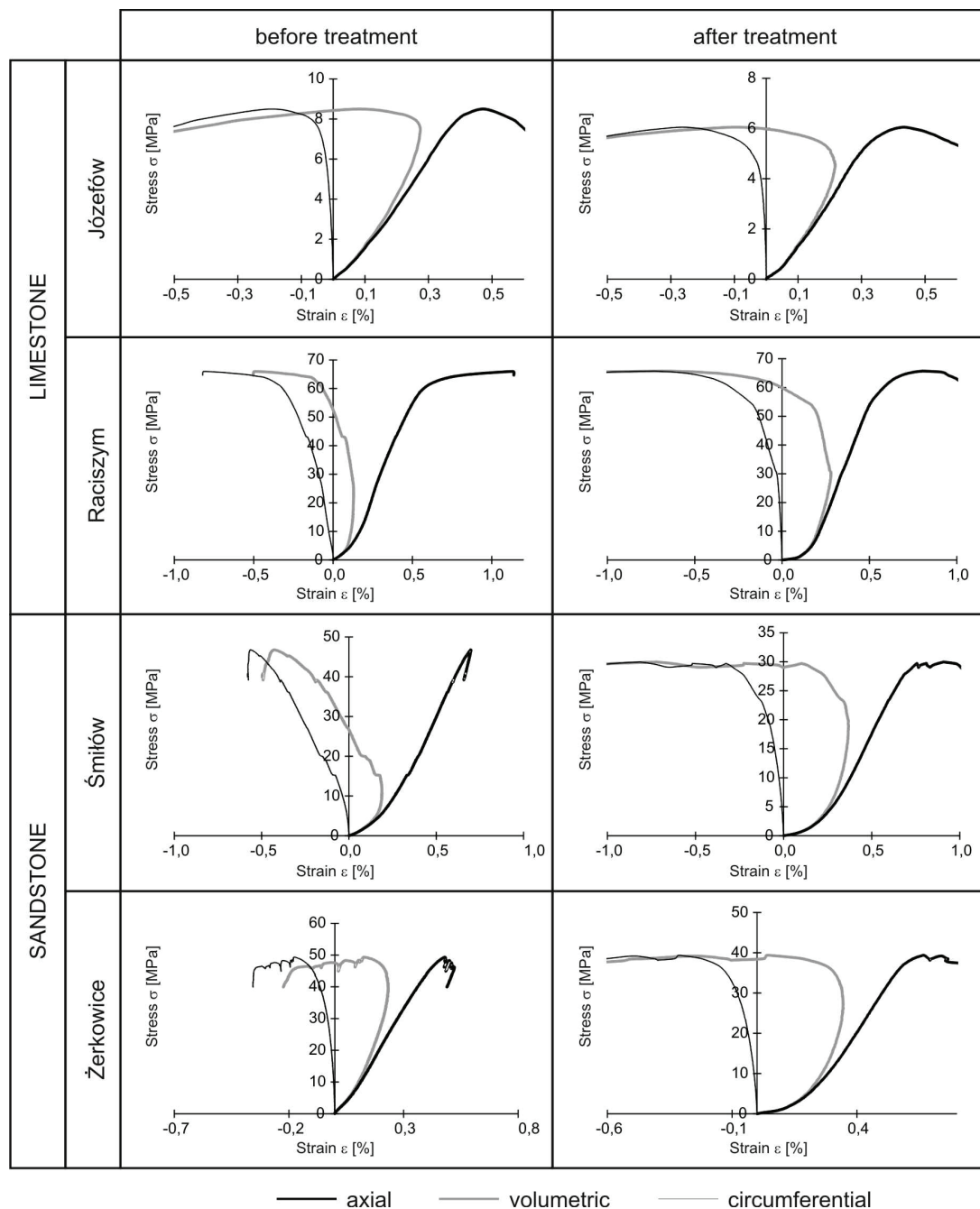
Fig. 9. Stress-strain characteristic of limestone from Józefów and from Raciszyn, sandstone from Śmiałów and from Żerkowice before and after the salt mist test
