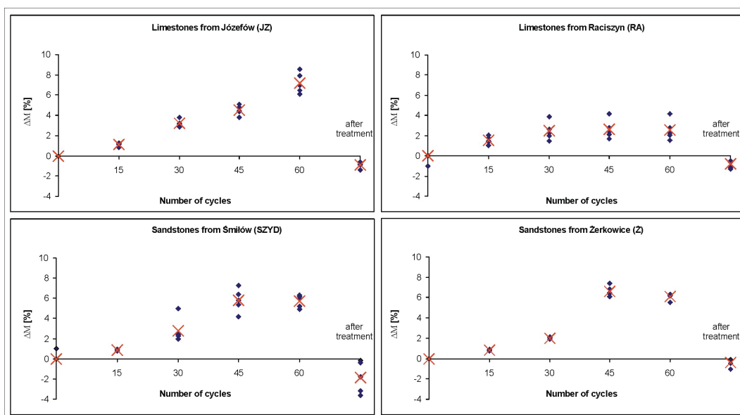
Fig. 7. Changes of weight during the test
