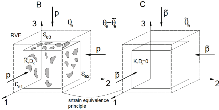
Fig. 5. Changes of the volumetric modulus of elasticity of the samples and the strain equivalence principle
