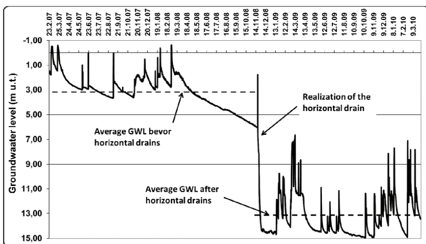
Fig. 5. Example of a decrease of GWL in observation well after the HDB realization
