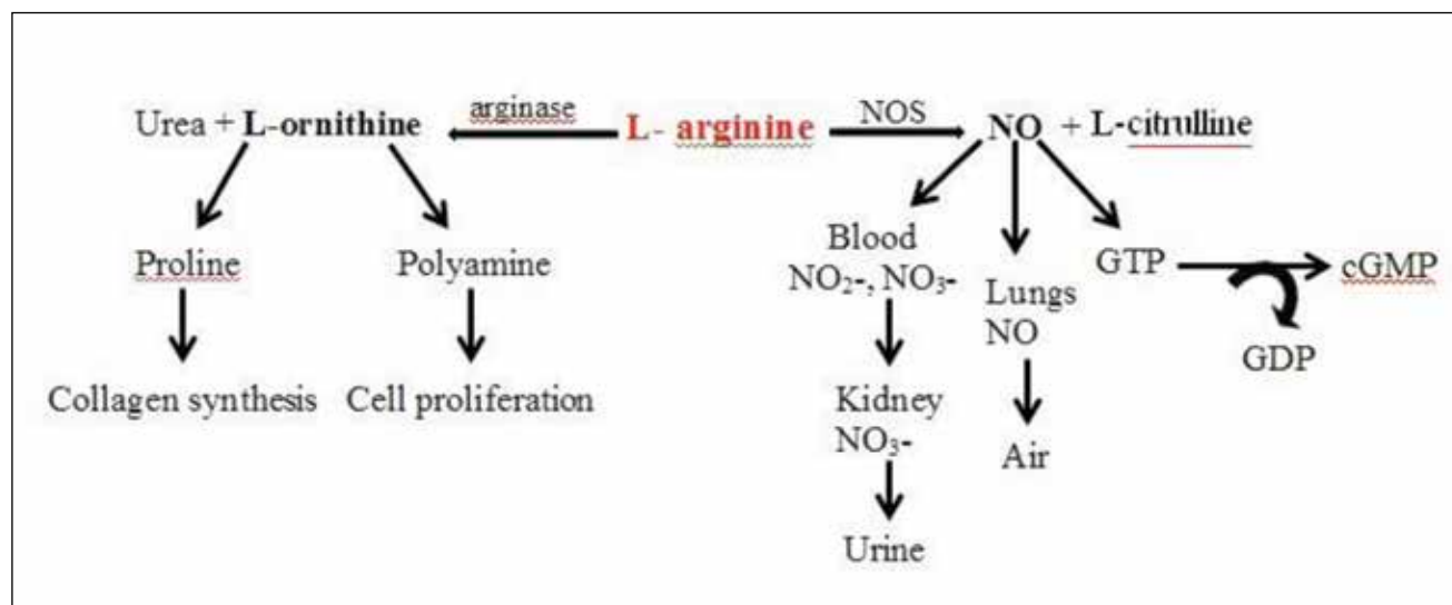
Figure 2 L-arginine pathways
