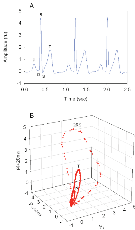
Figure 3. A. Registration of a single lead ECG data. B. Reconstruction of the three-dimensional activation of the /depolarization pattern/ as it could appear in a real system (heart). From Webber and Zbilut (2005) reprinted with permission
