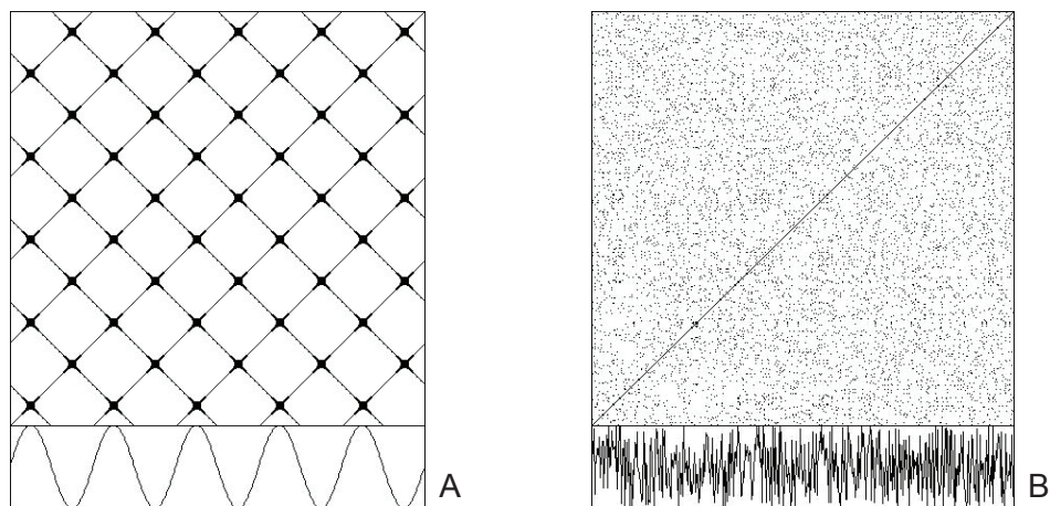
Figure 1. A. Sample time series of a sine function and its corresponding recurrence plot. B. Time series and corresponding recurrence plot of a white noise process. The lack of structure in the recurrence plot in B compared to the geometrical order of the recurrence plot of a deterministic time series (the sine function) in A is readily seen. Plots generated with the freely available program RQA Software v. 14.1 (by C. Webber Jr.)
