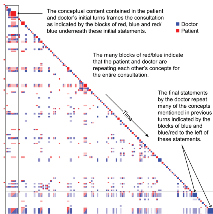
Figure 2. An example of conceptual recurrence plot of a conversation between doctor and patient. Recurrences are evident and some of its structure is indicative of significant synchronization / alignment in the interpersonal interaction. From Angus et al. (2012)
