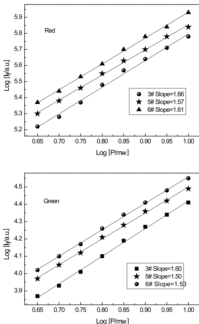
Figure 4. Pump power dependences of the green and red UC emission in \text{Yb}^{3+}/\text{Er}^{3+}/\text{GZO} ceramics
