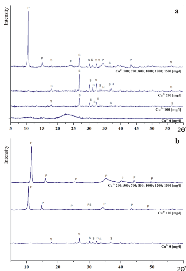
Fig. 2. Diffractometric analysis of residues from cultures on a Postgate C medium with (a) ethanol and (b) lactate as the sole carbon source. S, sulphur; P, pyrite; H, halite; PS, posnjakite
