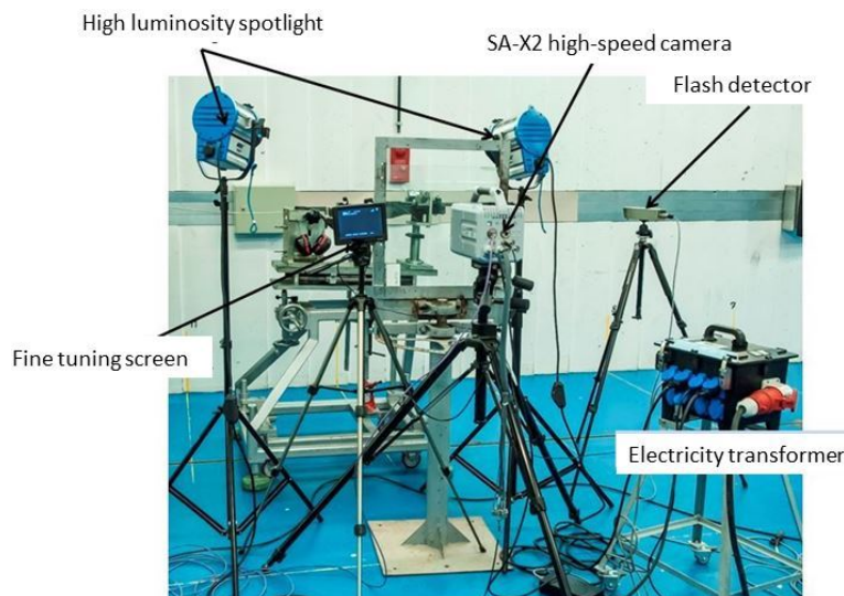
Figure 1: Barrel vibrations measuring chain
