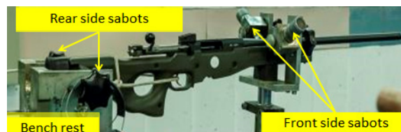
Figure 2: The way of fixing the firearm in a ruggedizing support (bench rest)
