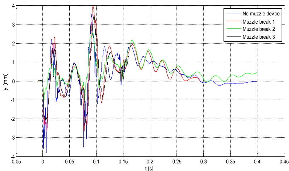
Figure: 5 Vertical displacement vs. time for the muzzle of a 5.56mm assault rifle with (a) no muzzle device, (b) muzzle device no 1, (c) muzzle device no 2, (d) muzzle device no 3 – 2 cartridges burst fire (e) Comparison between the vertical displacements of the muzzle
