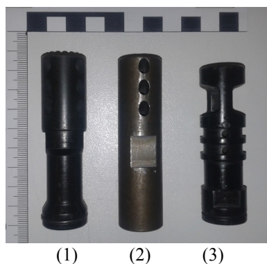
Figure 3: Muzzle devices used for firing with the 5.56mm assault rifle
