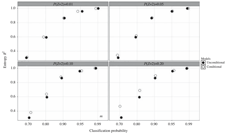
Fig. 2. Entropy R^2 of the unconditional and conditional model with different values for the classification probability and P(Z = 2) . The restricted conditional model has the same entropy R^2 as the conditional model because the models contain the same variables.
