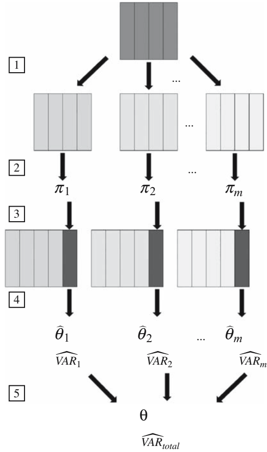
Fig. 1. Procedure of latent class multiple imputation for a multiply observed variable in a composite data set.
