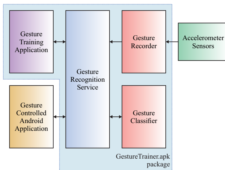
Fig. 2. Scheme of Android gesture recognition tool [15]
