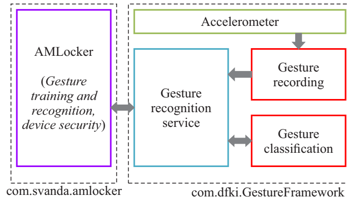
Fig. 3. Modified architecture of AMLocker
