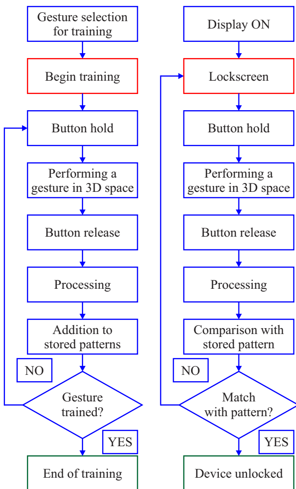
Fig. 4. Diagrams of training and unlocking process
