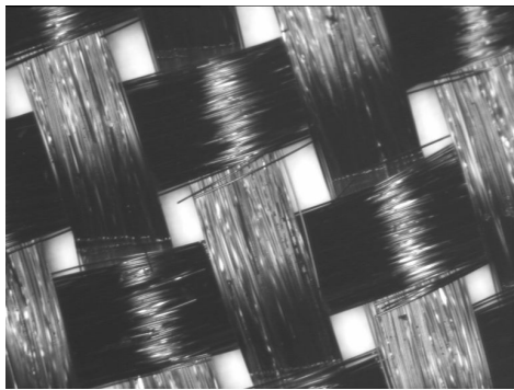
Fig. 5. Zoomed view of the textile's conductive carbon fibers [5]
