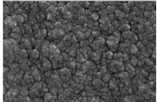
Fig. 6. SEM image of a rectangular sheet textile, layer thickness 1.2 microns, particles' size up to 50 nm (Reference: IOM Leipzig)
