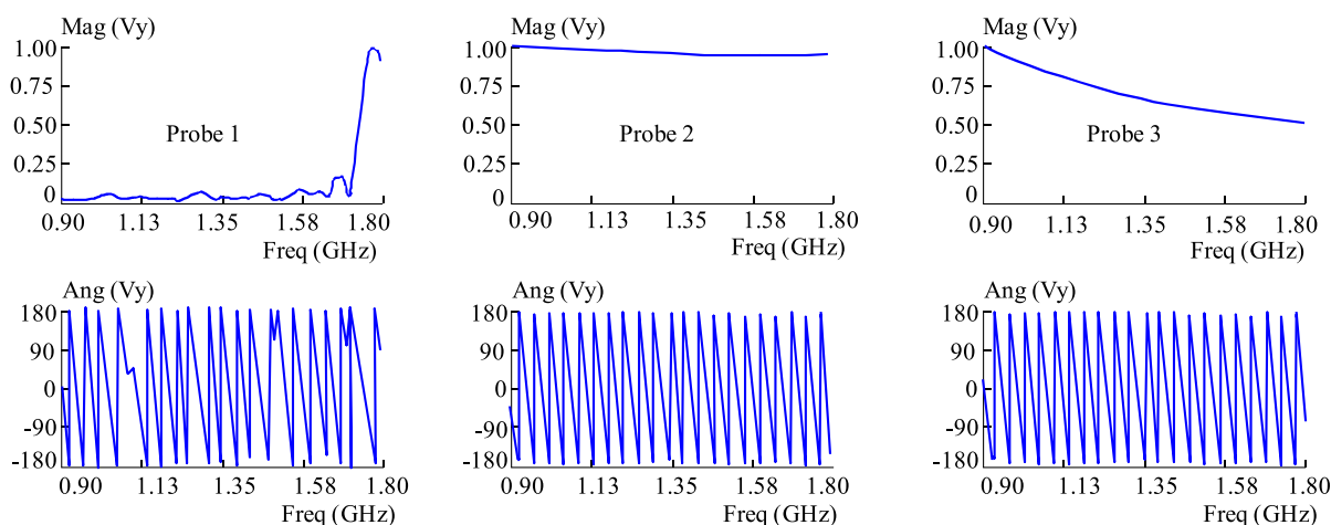
Fig. 13. Results for case 4 with both textile materials in graphs after the simulation [1]
