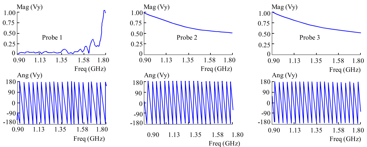
Fig. 11. Results for case 2 with nanoferrite textile shielding in graphs after the simulation [1]
