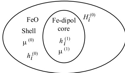
Fig. 7. Construction of a magnetic nanoparticle with magnetic fields acting [5], h_i^{(1)} – dynamic magnetic field, H_z^{(0)} – static magnetic field, \mu^{(1)} – internal permeability, \mu^{(0)} – external permeability
