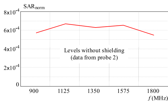
Fig. 15. Levels of SAR_{norm} in frequency range f = 0.9 to 1.8 GHz without shielding
