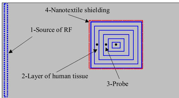
Fig. 10. View of the simulation area in the cases with shielding materials (enclosed shielding around the head) [1]
