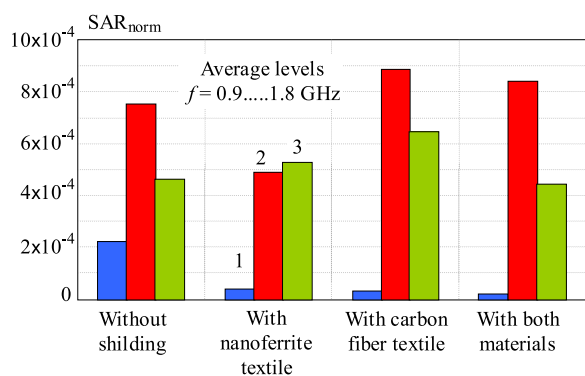
Fig. 14. Average levels of SAR_{norm} in frequency range f = 0.9 to 1.8 GHz: 1 probe under the skin, 2 probe under the muscle tissue, 3 probe inside the brain
