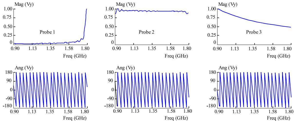
Fig. 9. Results for case 1 without shielding in graphs after the simulation [1]
