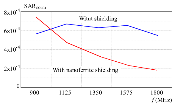
Fig. 17. Levels of SAR_{norm} in frequency range f = 0.9 to 1.8 GHz with nanoferrite textile
