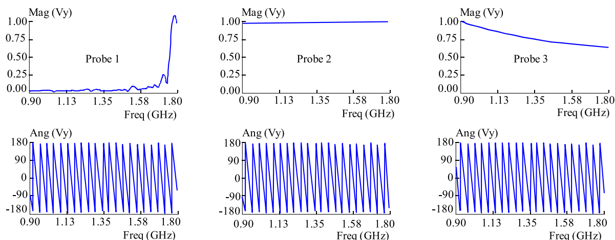
Fig. 12. Results for case 3 with carbon fiber textile shielding after the simulation [1]
