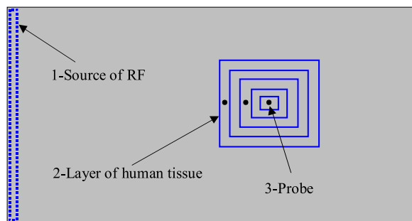
Fig. 8. View of the simulation area in case 1 – no shielding [1]
