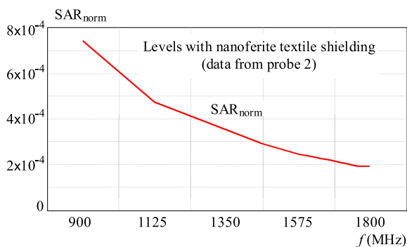
Fig. 16. Levels of SAR_{norm} in frequency range f = 0.9 to 1.8 GHz with nanoferrite textile
