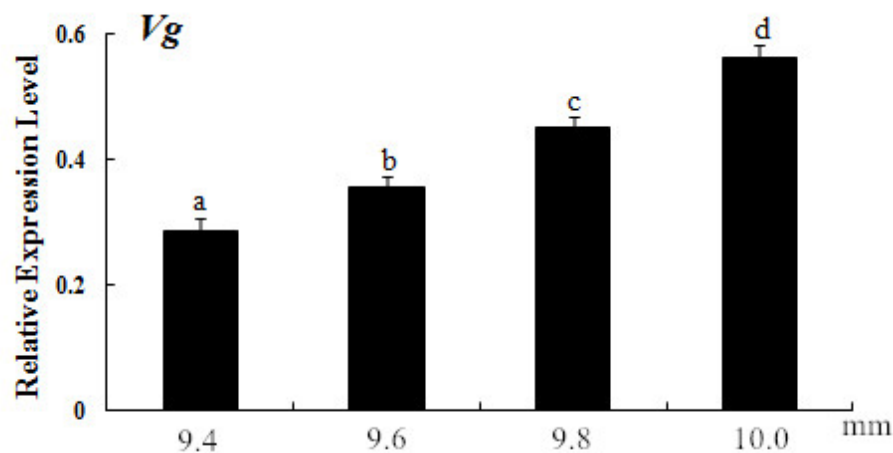
Fig. 2 Effect of queen cell diameter on gene expression of Vg in queen's ovarian tissues. Histogram shows the relative Vg expression level. Each bar corresponds to a single group and shows the mean \pm SE of three biological replicates. N=9. Different letters above bars mean a significant difference between groups ( P < 0.05 ). The same as below.
